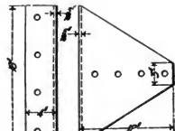
Figs. 4175-4176. Back Brace Plate.
